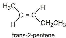
trans-2-pentene
