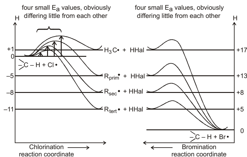
Figure : Thermochemical analysis of that propagation step of radical chlorination (left) and bromination (right) of alkanes that determines the regioselectivity of the overall reaction. The H^\ddagger values were determined experimentally; the DH^{++} values are estimated
