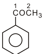
1-phenylethan-1-one (Acetophenone or methyl phenyl ketone)
