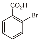
2-bromobenzoic acid
