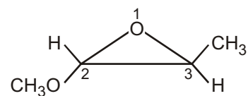
trans-2-methoxy-3-methyloxirane 1,2-epoxy-1-methoxypropane
