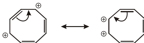
the charges can be delocalized all round the ring
