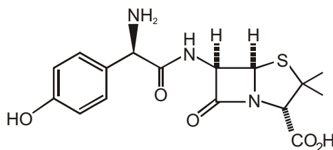
Smith Kline Beecham's amoxycillin \beta -lactam antibiotic for treatment of bacterial infections
