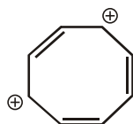
one structure with localized charges
