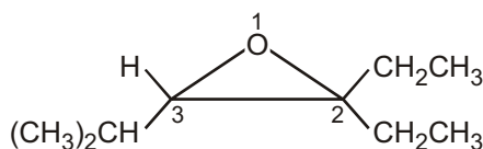
2,2-diethyl-3-isopropylloxirane 3,4-epoxy-4-ethyl-2-methylhexane
