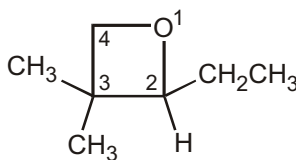
2-ethyl-3,3-dimethyloxetane
