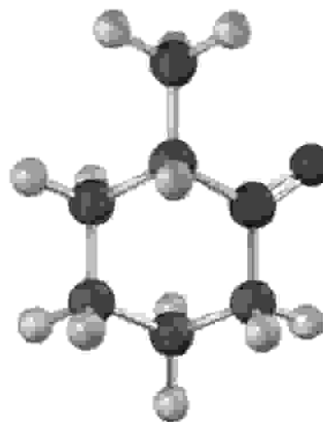
2-Methylcyclohexanone (chiral)
