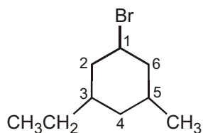
1-Bromo-3-ethyl-5-methyl cyclohexane
