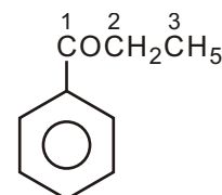
1-phenylpropan-1-one (Propiophenone)
