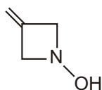
alkene, secondary amine, alcohol (cyclic hydroxylamine)
