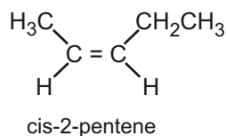
cis-2-pentene
