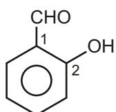
2-hydroxybenzaldehyde (salicylaldehyde)
